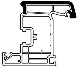
80mm INSWING SASH 103.232
