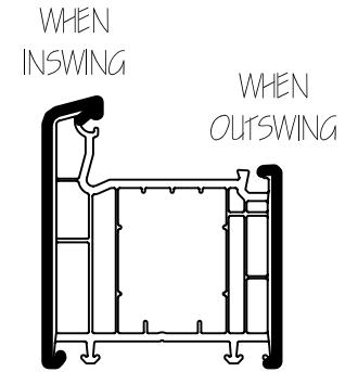
80mm MAINFRAME 101.214
