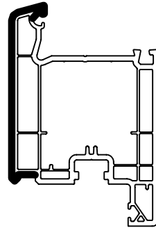
105mm INSWING SASH 103.241
