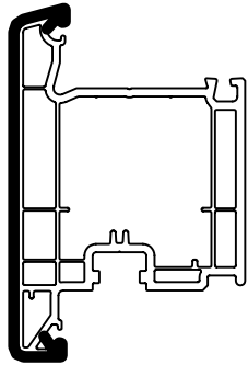
105mm OUTSWING SASH 103.242
