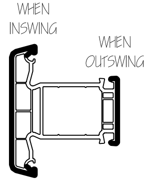
85mm T-MULLION 102.218
